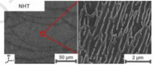
Microstructure without heat treatment (NHT)
